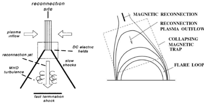
Fig. 13 Left , cartoon showing the current sheet and associated processes invoked as the core of the standard model (Cargill 2001). However such processes can occur at current sheets with a wide range of scales. In particular island formation, as illustrated in Figure 15, could take place within the current sheet. Right , a sketch of the collapsing magnetic trap (Karlický and Kosugi 2004).
