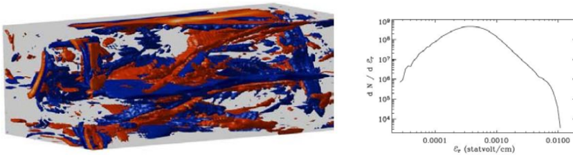
Fig. 14 Left : Snapshot of the resistive electric field configuration inside a coronal loop driven by random motions of the magnetic footpoints at the left and right faces of the simulation box; and right : the distribution of electric field strength seen by a typical particle traveling inside this “loop.” The red and blue indicate fields pointing towards opposite faces of the box. From Turkmani et al (2006).
