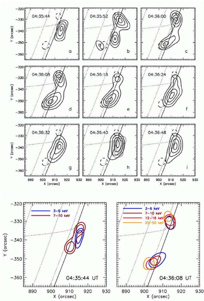
Fig. 5 Upper: RHESSI 3-6 keV maps of the 28 November 2002 flare, showing the apparent motions upwards along a loop; the 25-50 keV contour image (dashed contours) at the hard X-ray peak time is overlaid in each panel. Lower: spectrally-resolved images showing the footpoint locations more clearly. The solid curves in all panels show the solar limb, while the dotted curves show heliographic parallels and meridians.
