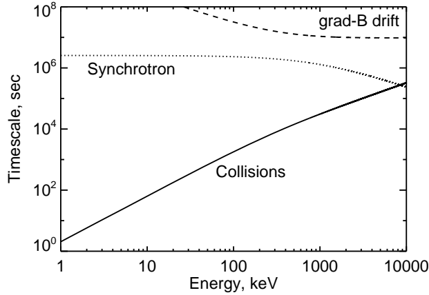
Fig. 16 Representative time scales for fast electrons in the solar corona: solid, the Coulomb collision time assuming a density of 10^8 \text{ cm}^{-3} ; dotted, synchrotron radiation assuming B = 10 \text{ G} ; dashed, gradient-B drift over a spatial scale of 0.1 R_{\odot} .
